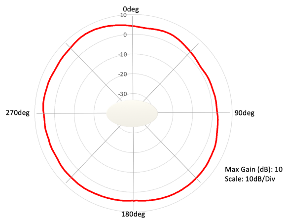
2.4 GHz Azimuth
